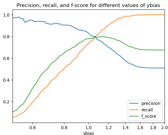
Figure 1: Metrics for different values of ybias in one of the fine-tuned SBERT models
